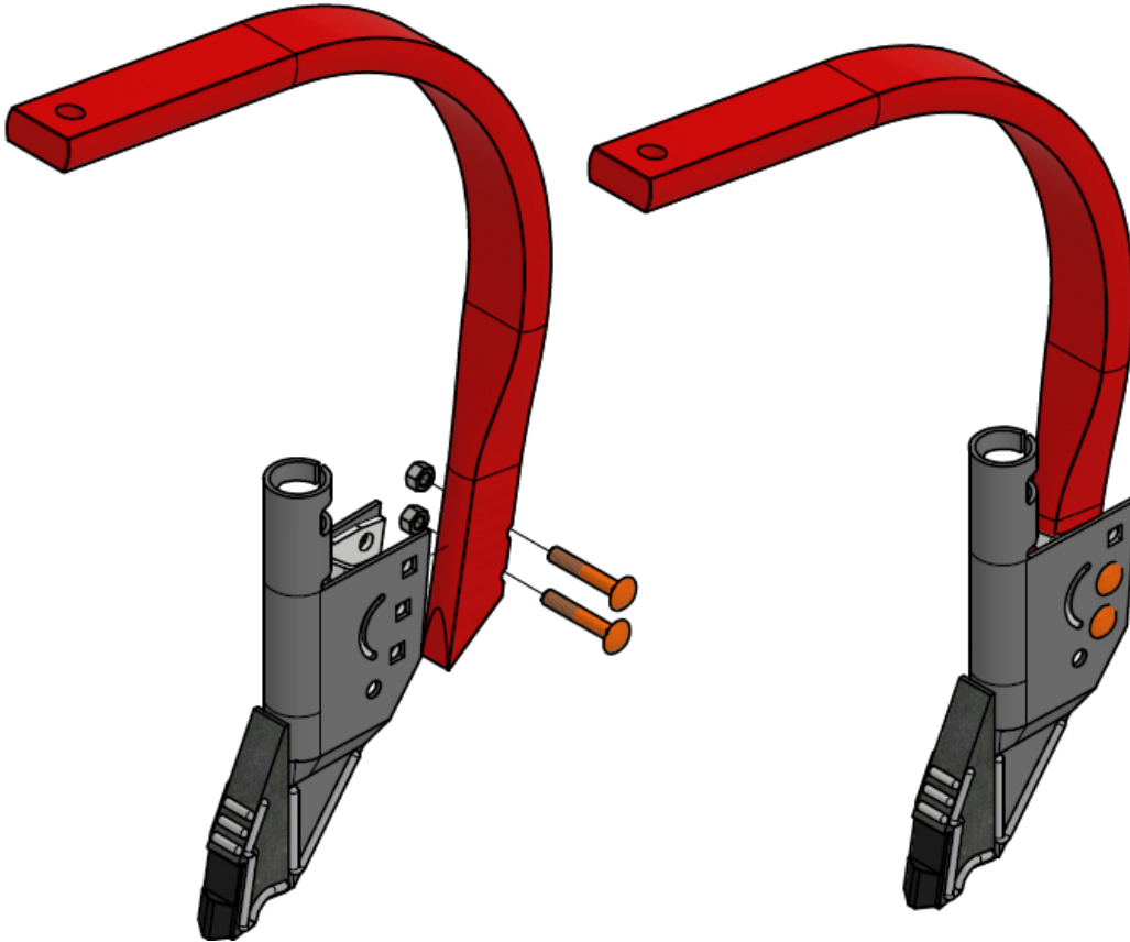
Figure 1: Bolt opener to shank
