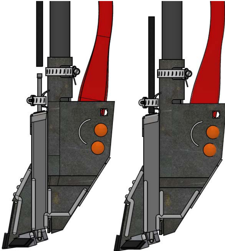
Figure 6: Install fertilizer hose
