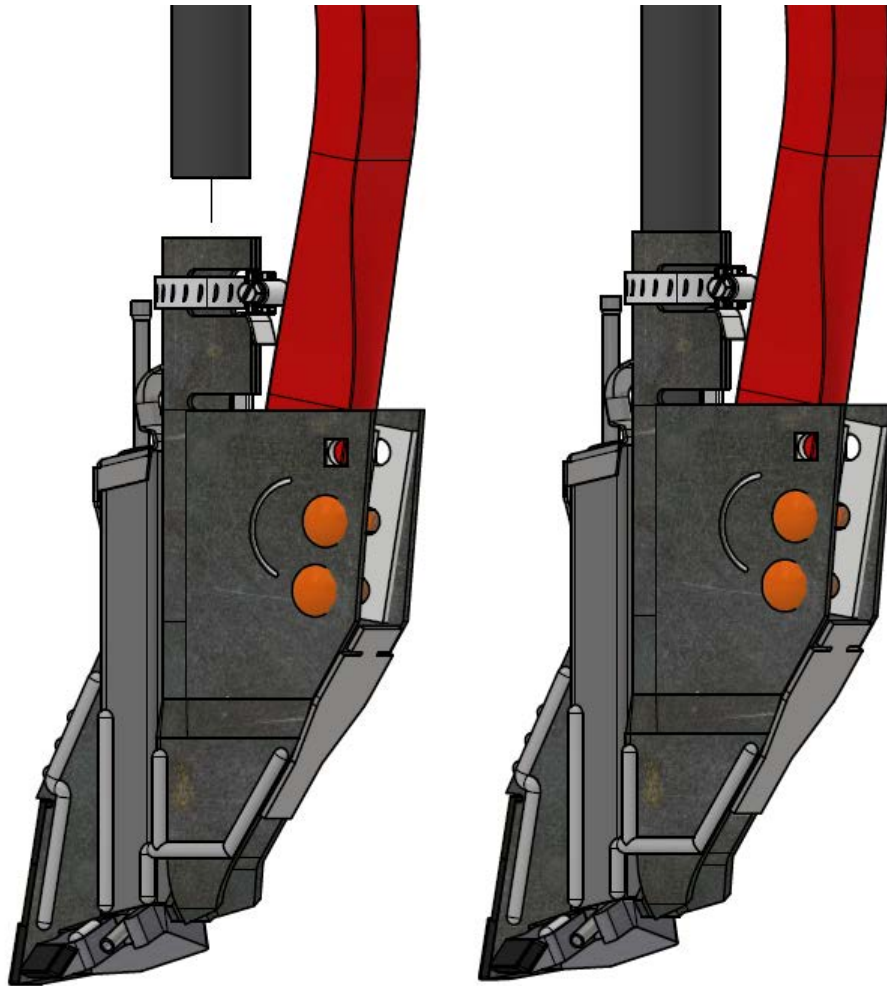
Figure 5: Install seed hose
