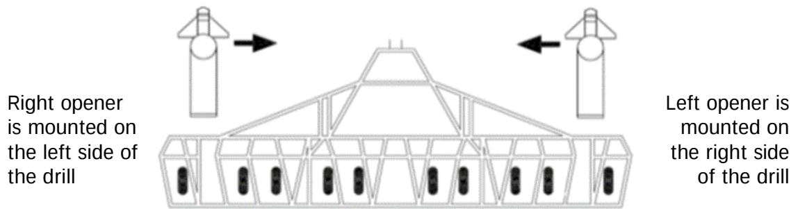
Figure 3: Opener orientation
