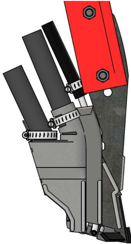
Figure 10: Installed protective tube
