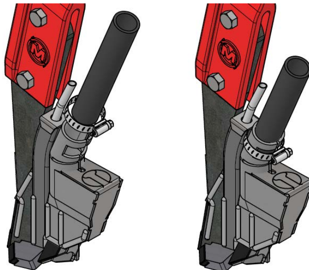
Figure 5: Install dry tube for single shoot set up
