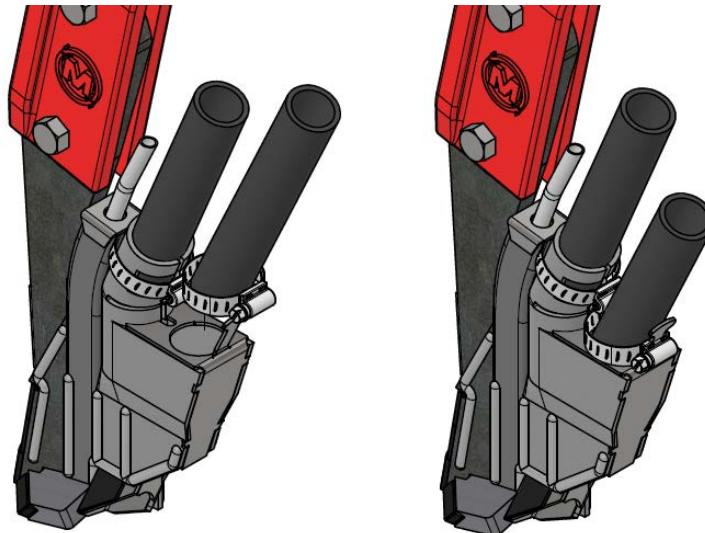
Figure 6: Install tubes for double shoot dry set up
