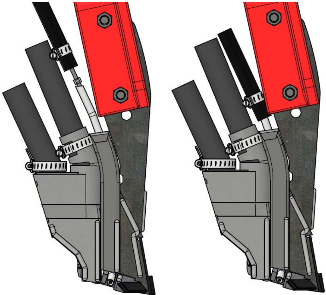
Figure 12: Install protective cover over MaxQuip line
