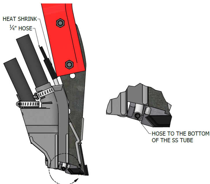
Figure 9: Install ¼" NH3 line
