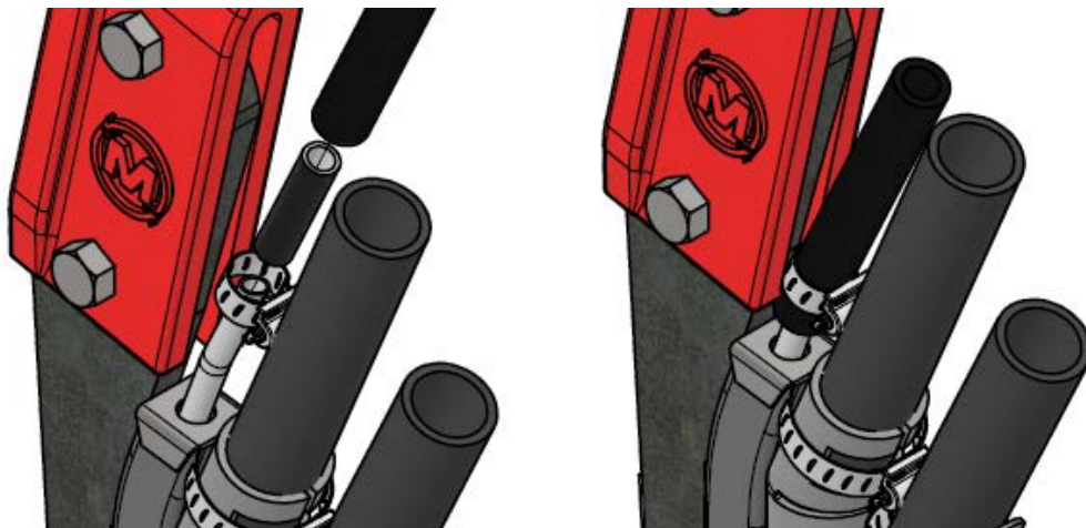
Figure 8: Install ½" NH3 line
