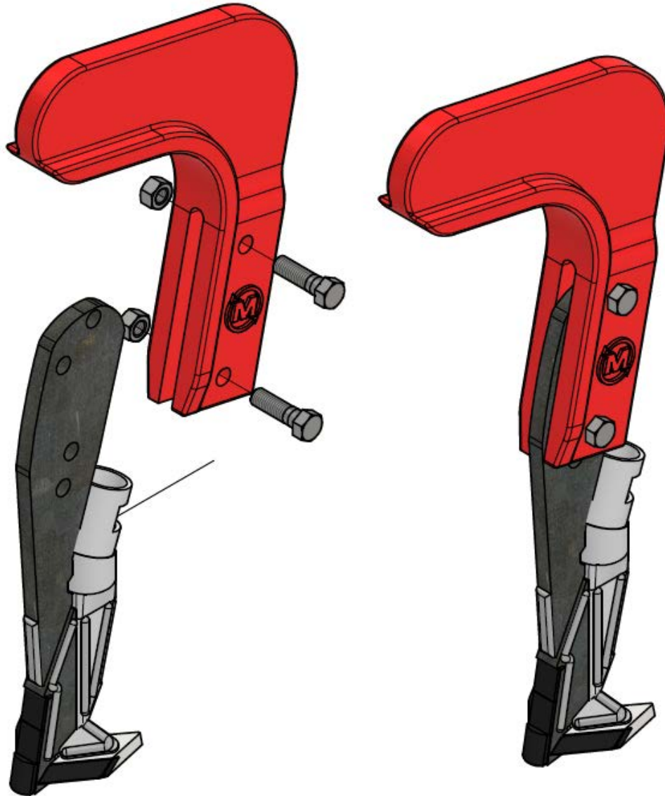
Figure 2: Bolt opener to shank
