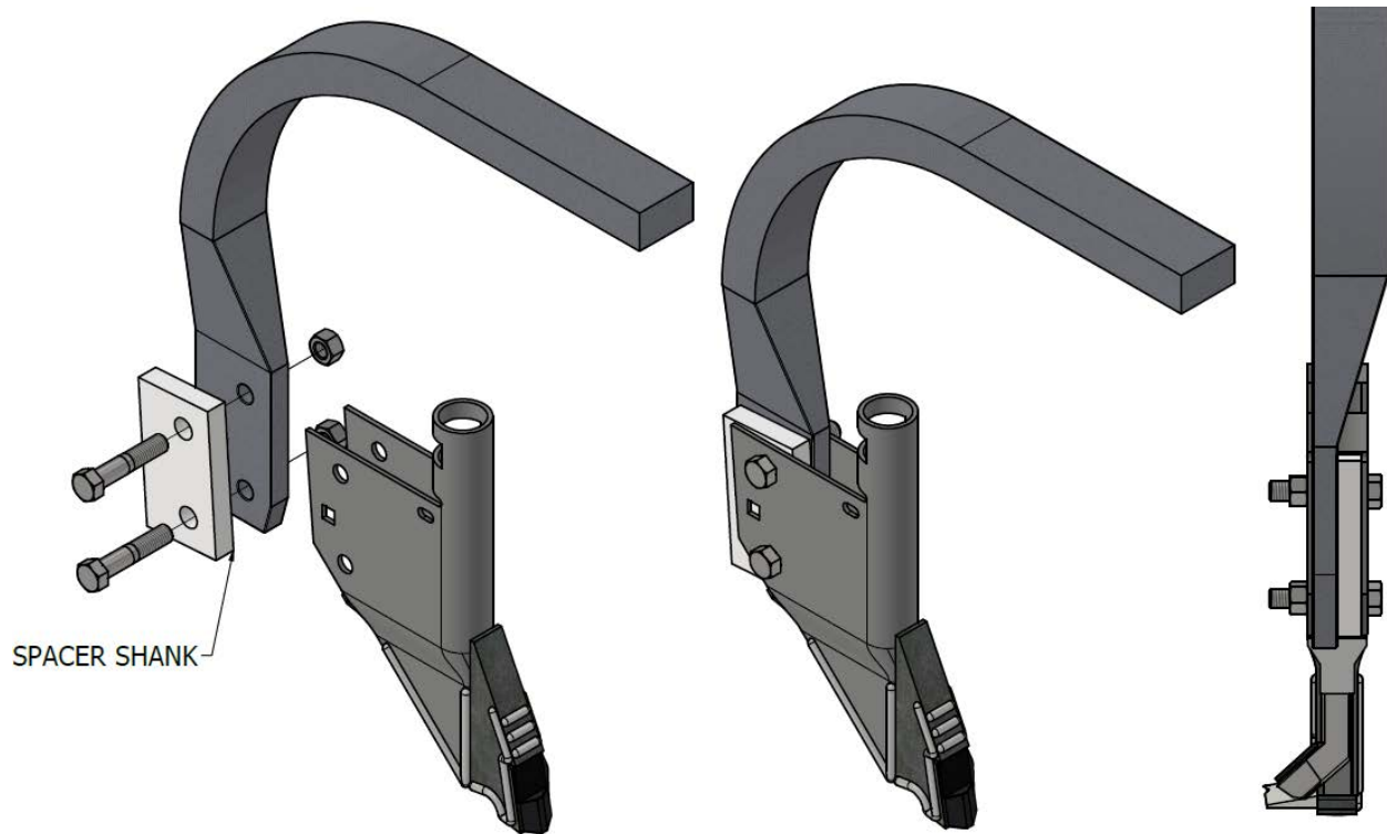
Figure 1: Bolt opener to shank
