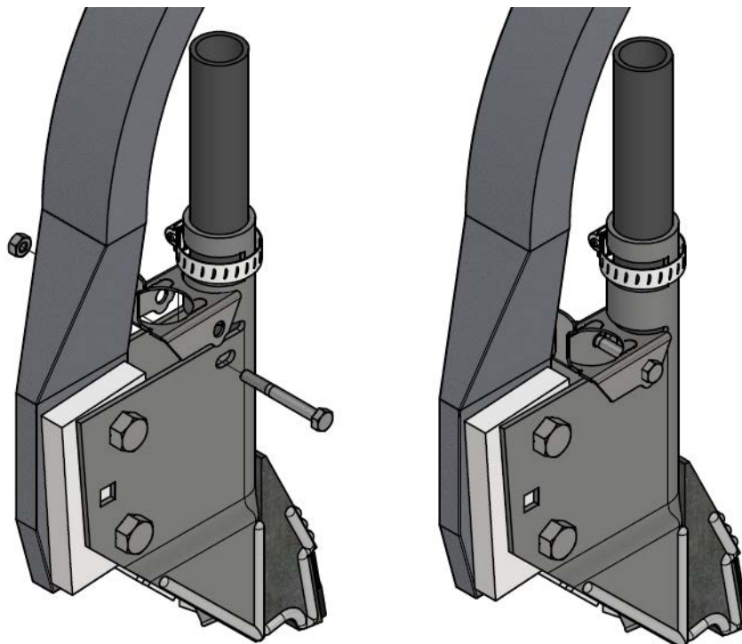
Figure 4: Install opener top
