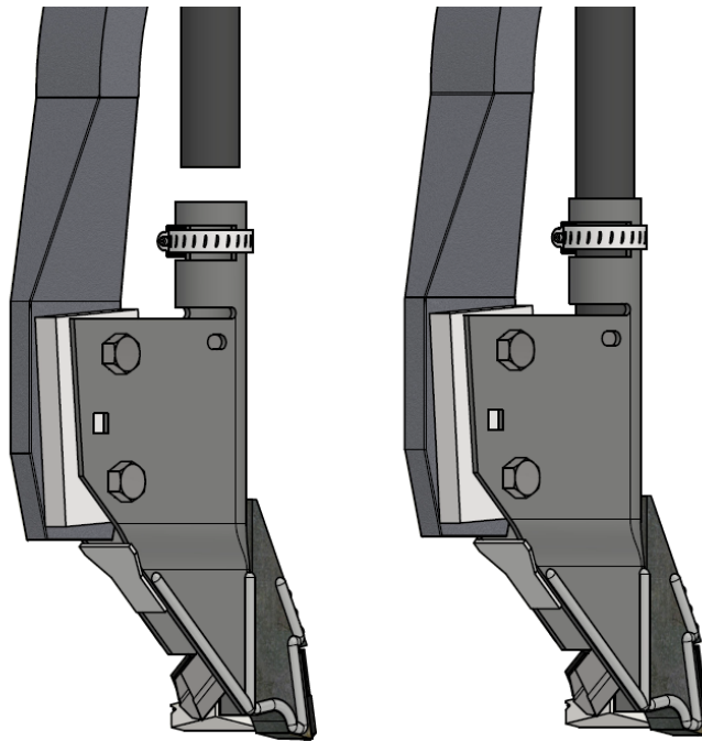
Figure 3: Install front dry hose
