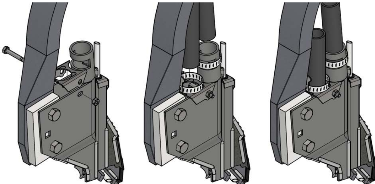
Figure 6: Install tubes for double shoot dry set up
