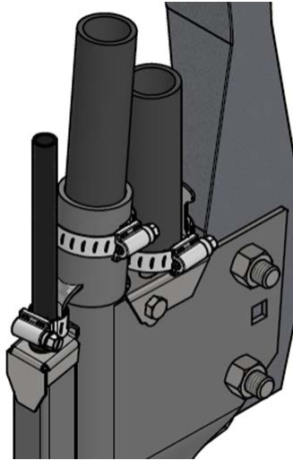
Figure 7: Install \frac{3}{8} " NH3 line
