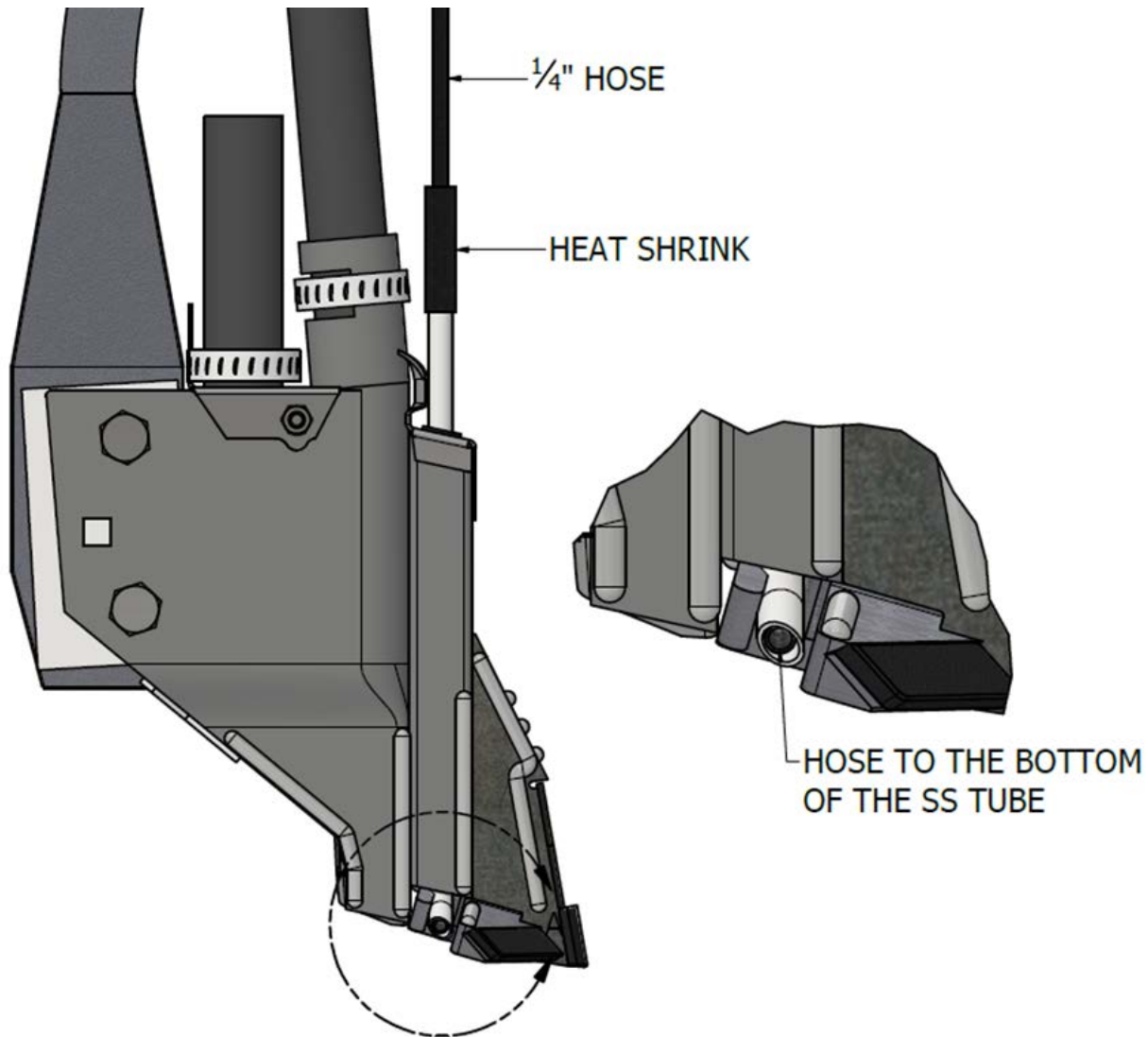
Figure 9: Install 1/4" NH3 line
