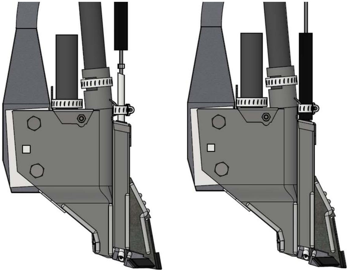
Figure 12: Install protective cover over MaxQuip line
