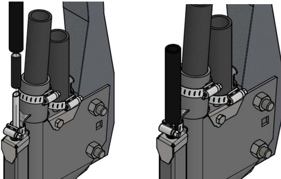
Figure 8: Install \frac{1}{2} " NH3 line
