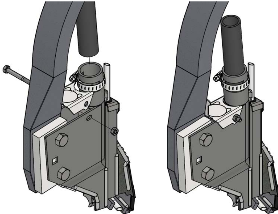
Figure 5: Install dry tube for single shoot set up
