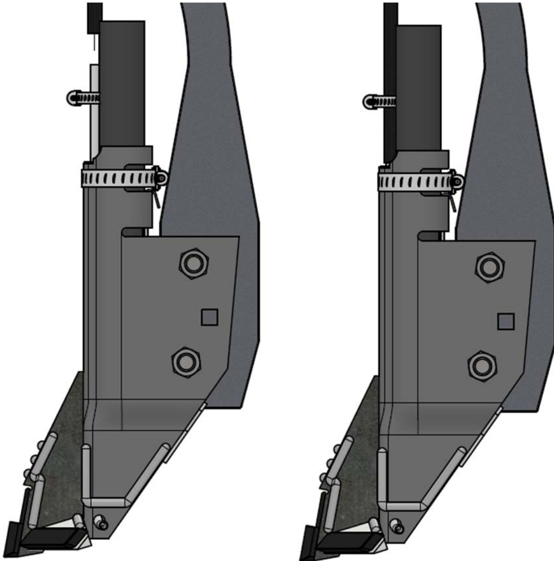
Figure 8: Install liquid fertilizer tube
