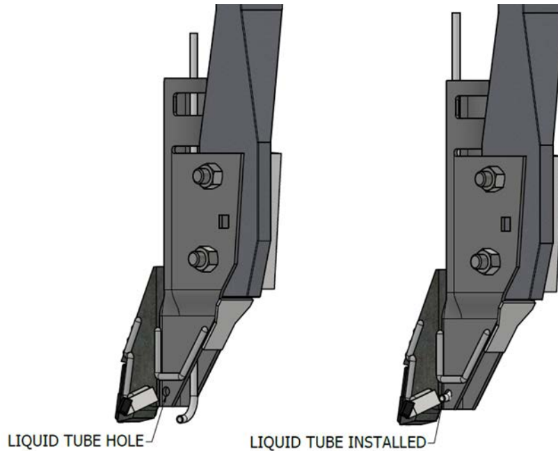
Figure 4: Install liquid tube
