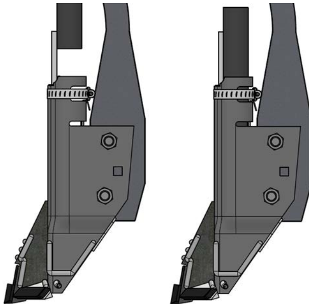
Figure 7: Install seed tube
