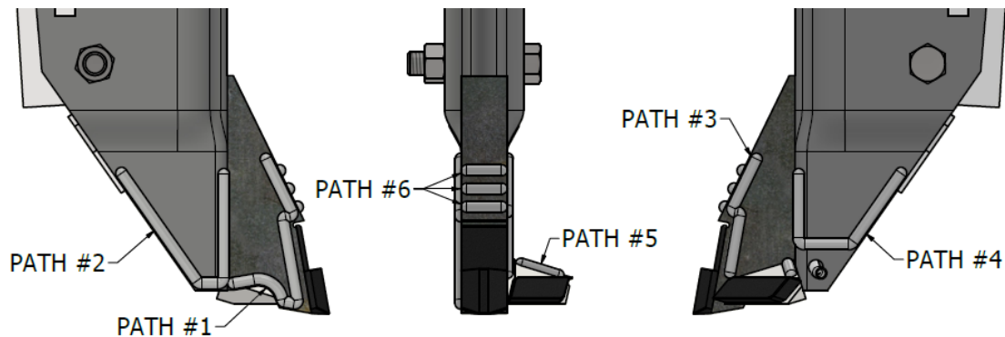
Figure 9: Hard surface paths
